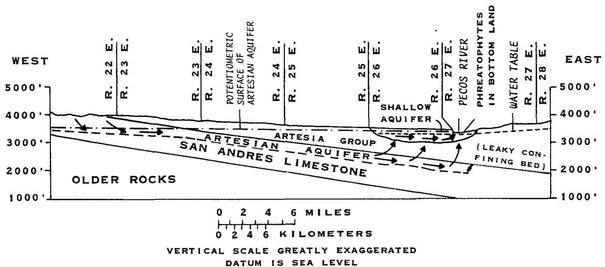
Figure 3.--Generalized geohydrologic section showing relation of the aquifers of the Roswell ground-water basin to the Pecos River and direction of ground-water flow.
