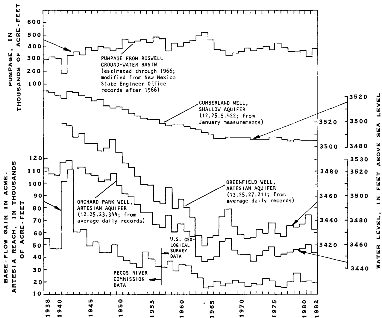
Figure 4.--Relation of annual pumpage from the Roswell ground-water basin, hydraulic heads in the shallow and artesian aquifers, and base-flow gain of the Acme-Artesia reach, 1938-82.
