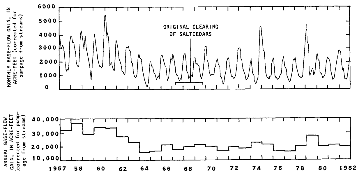
Figure 9.--Monthly and annual base-flow gain in the Acme-Artesia reach, 1957-82.
