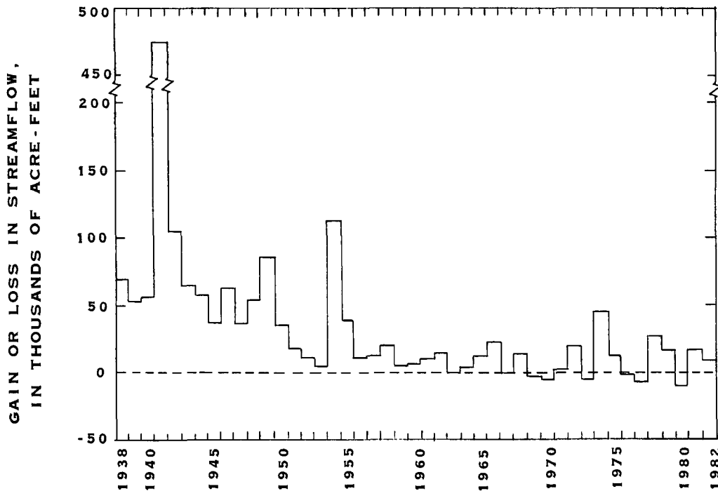
Figure 2.--Difference in streamflow of the Pecos River between the Acme and Artesia streamflow-gaging stations, 1938-82 (prepared from streamflow discharge records collected by the U.S. Geological Survey).
