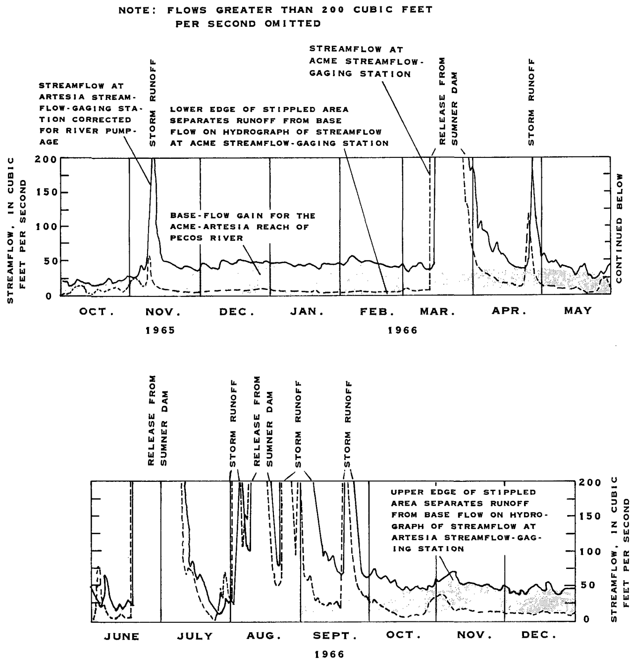
Figure 8.--Method of separating base flow on streamflow hydrographs of the Acme and Artesia streamflow-gaging stations (modified from Welder, 1973, fig. 3).
