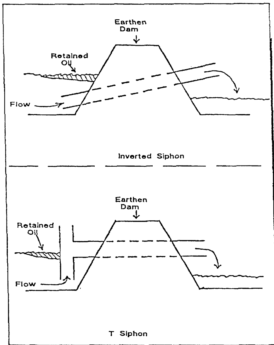
Figure D-5. Earthen Dam Construction.
