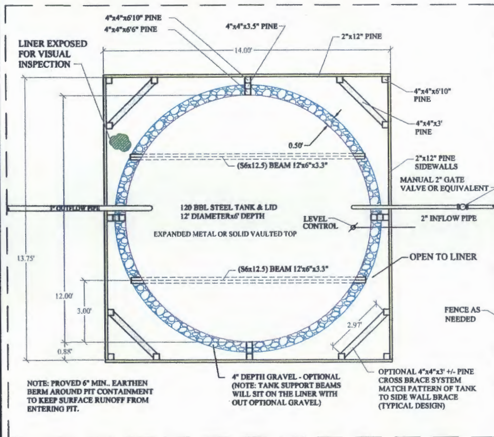
PLAN VIEW
