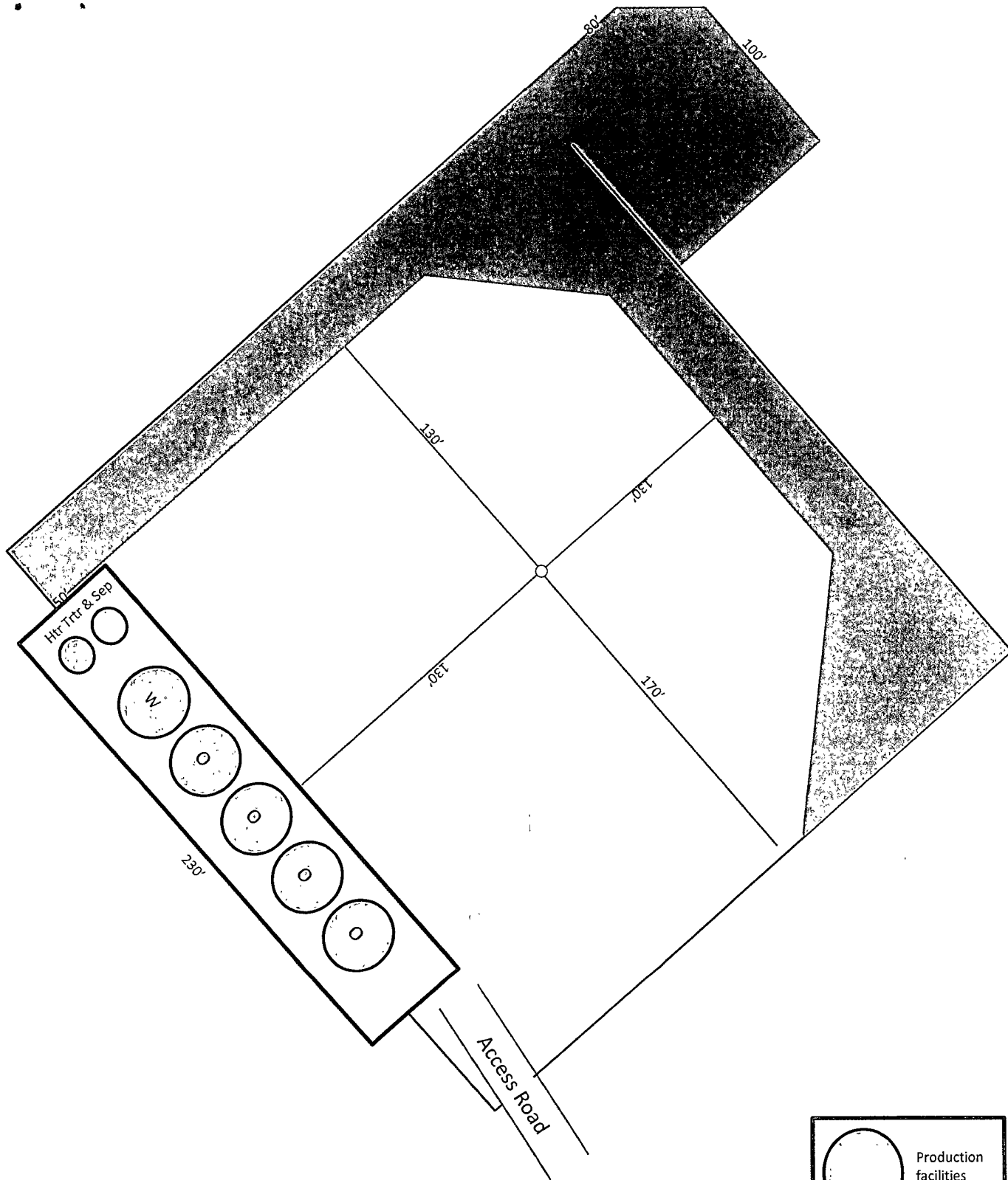
Exhibit D-1 Production Facilities Layout Diagram Southeast Lusk 33 Federal No. 2 Cimarex Energy Co. of Colorado 33-19S-32E SHL 530 FNL & 737 FEL BHL 330 FSL & 660 FEL Lea County, NM
