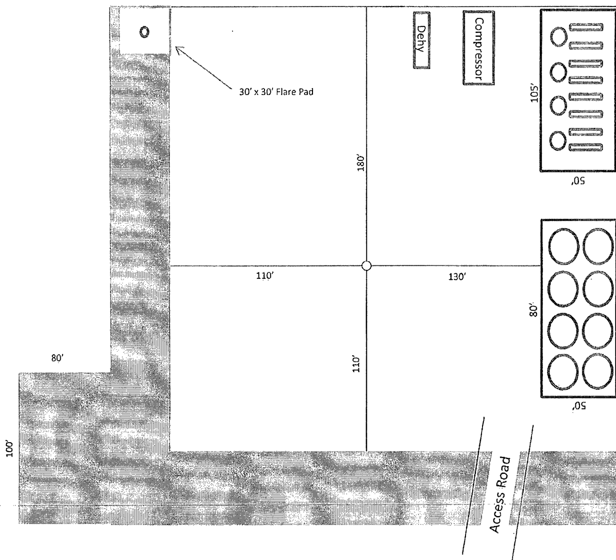
Exhibit D-1 Production Facilities and Interim Reclamation Diagram West Grama Ridge 6 Federal #4H Cimarex Energy Co. of Colorado SHL 6-22S-34E; 330 FNL & 660 FEL BHL 6-22S-34E; 330 FSL & 660 FEL Lea County, NM
