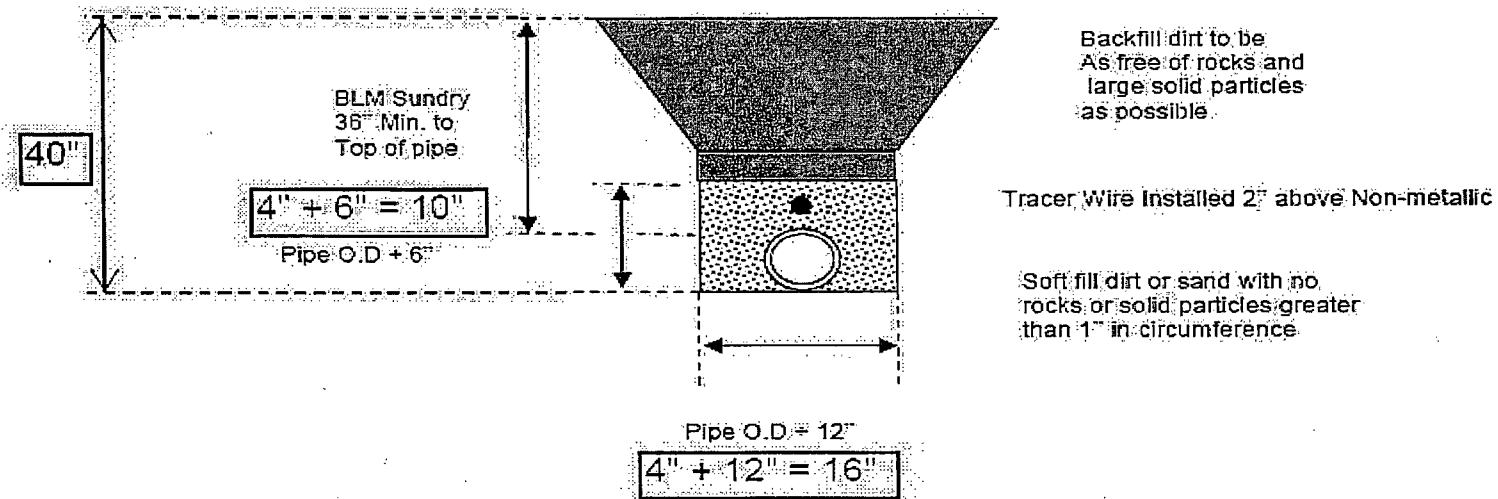
Figure D-1 Backfill around Pipe
