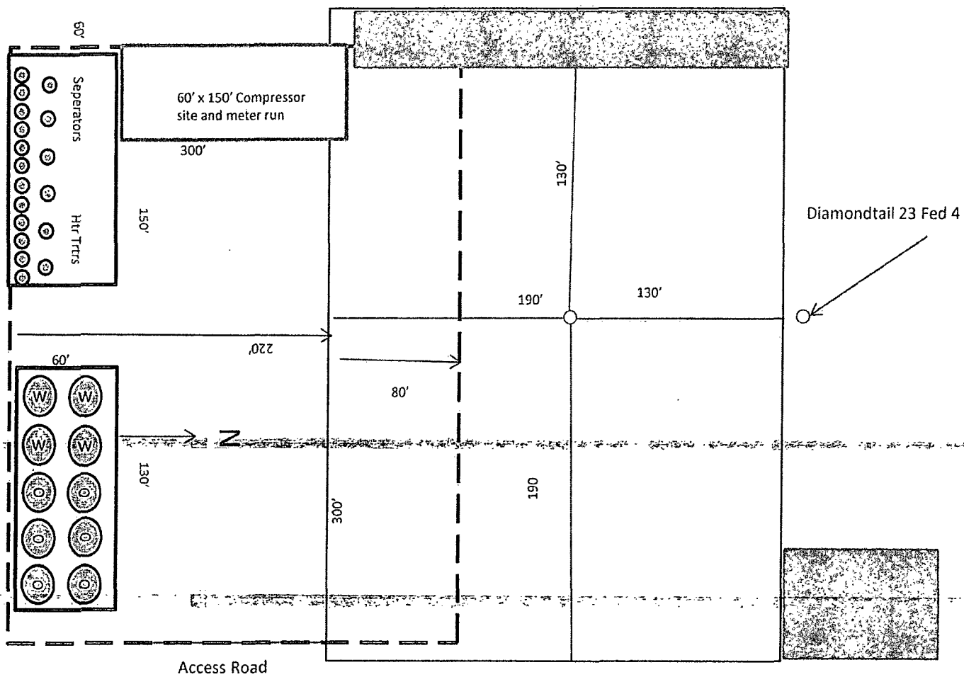
Exhibit D-1 Production Facilities Layout Diagram Diamondtail 23 Federal 3 Cimarex Energy Co. 23-23S-32E SHL 330 FNL & 1805 FWL BHL 330 FSL & 1650 FWL Lea County, NM
