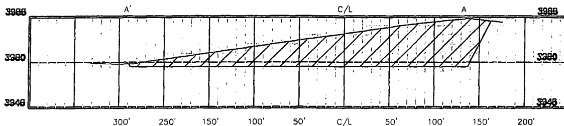
"A" (NORTH) PROFILE
