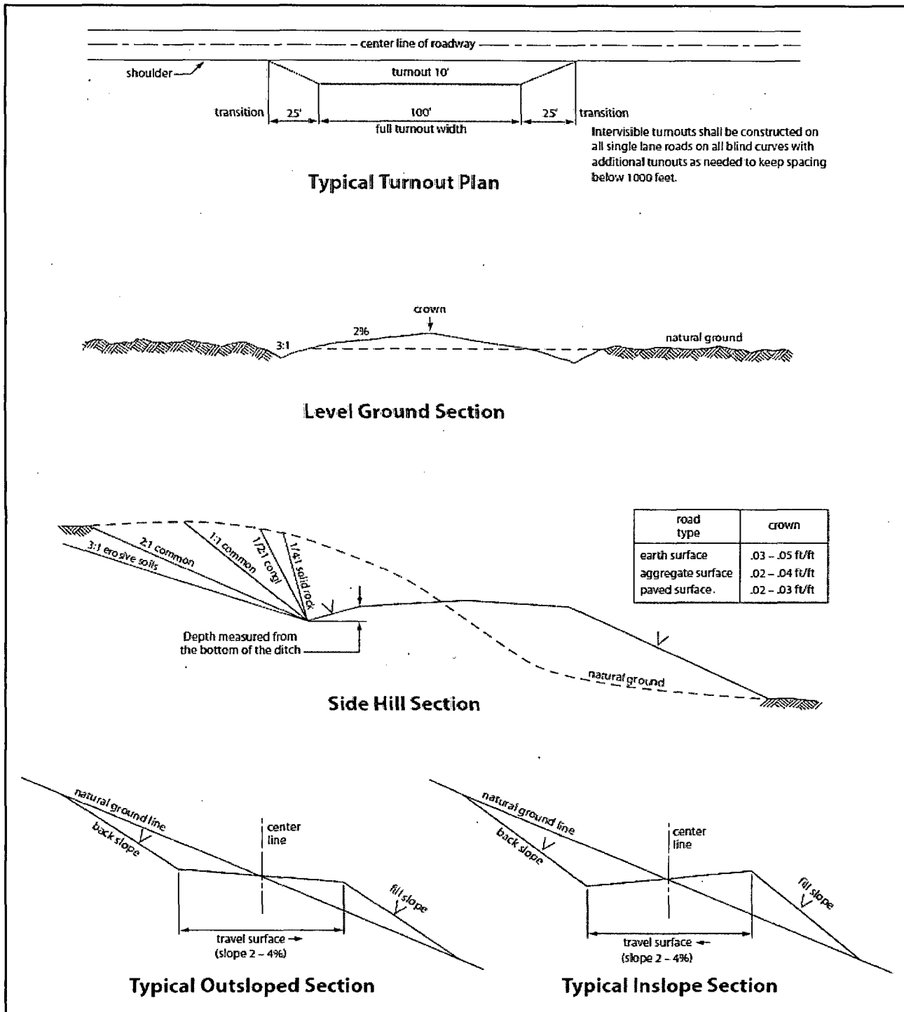
Figure 1. Cross-sections and plans for typical road sections representative of BLM resource or FS local and higher-class roads.
