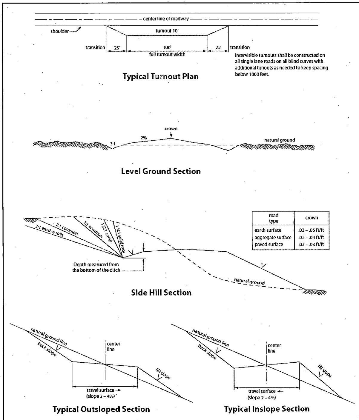
VII. Figure 1. Cross-sections and plans for typical road sections representative of BLM resource or FS local and higher-class roads. DRILLING
