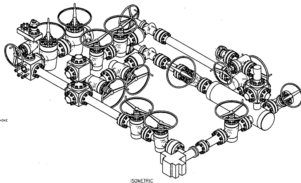
ISOMETRIC
