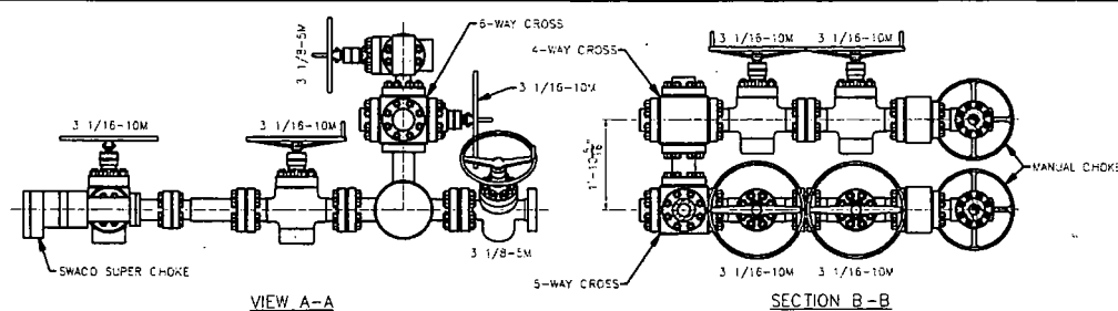
SECTION B-B
