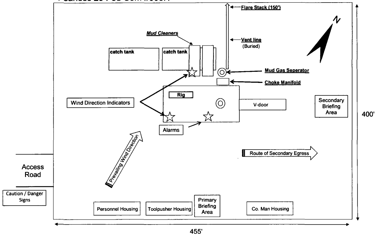
Well Site Diagram
