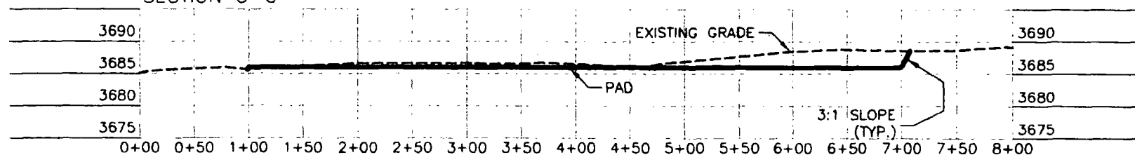
SECTION C-C'
