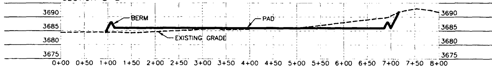
SECTION B-B'
