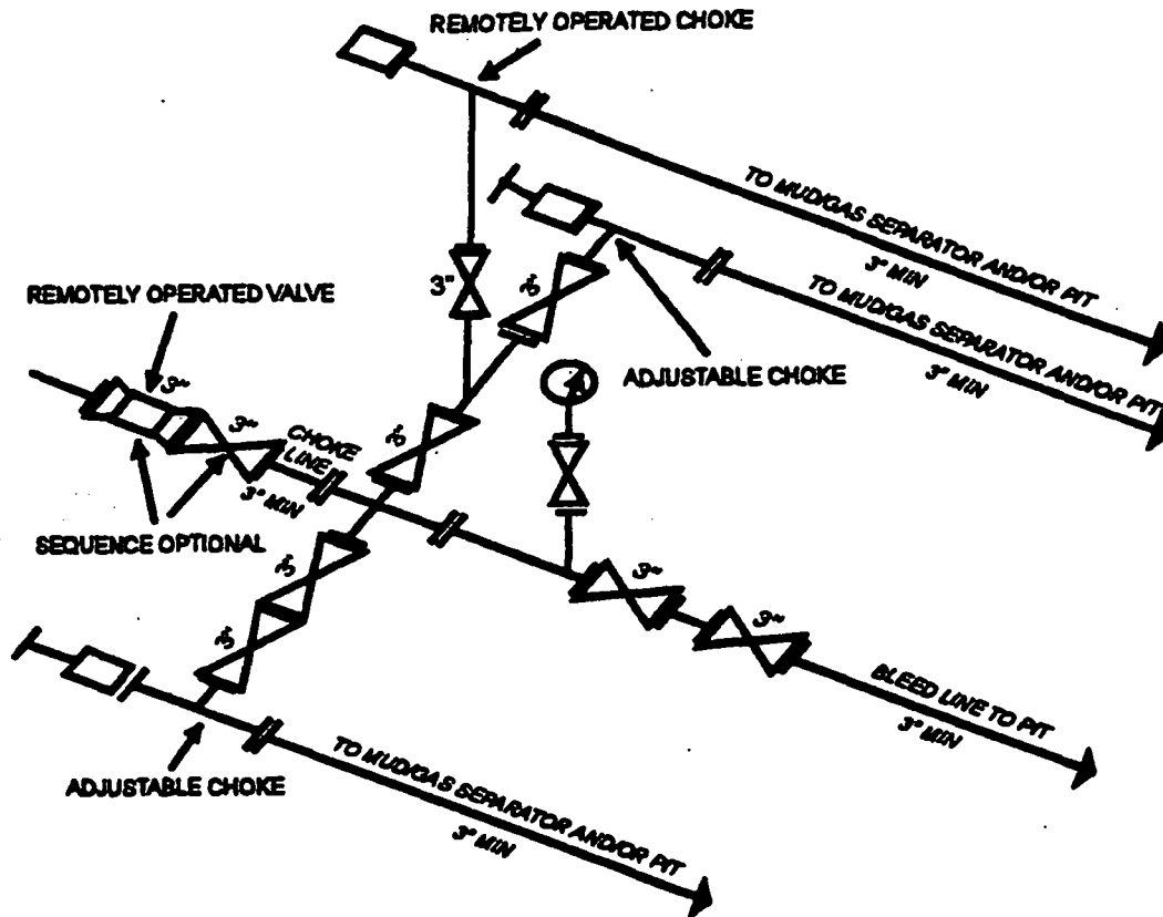
10M AND 15M CHOKE MANIFOLD EQUIPMENT - CONFIGURATION OF CHOKES MAY VARY [33 FR 49661, Dec. 9, 1968 and 54 FR 39528, Sept. 27, 1989]
