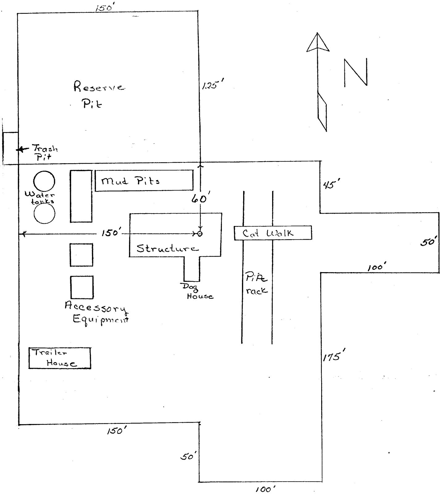
Exhibit "C" Patterson Fed #1 Sec 4, T19S, R32E Lea Co., New Mexico Drilling Pad layout
