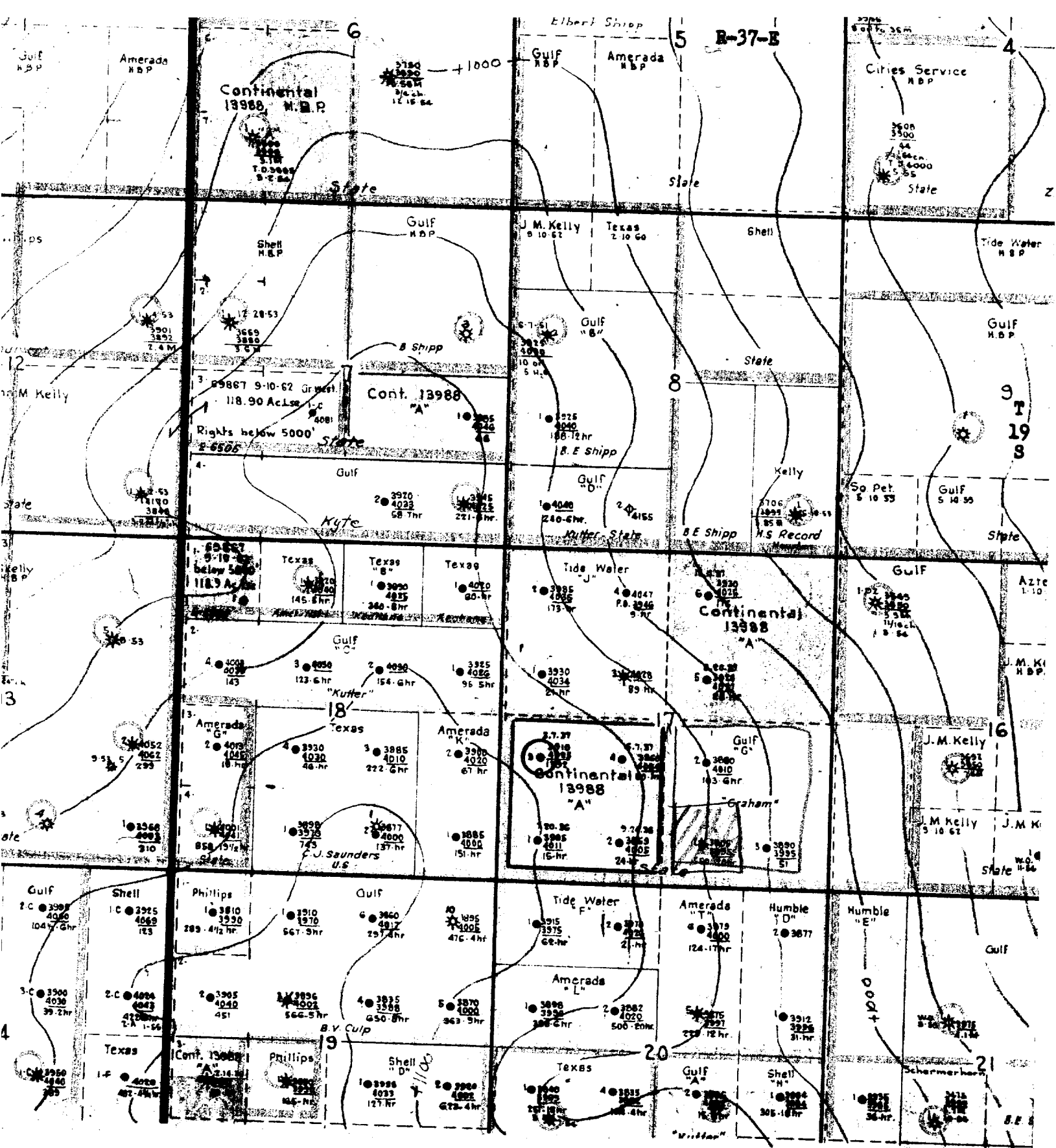
STRUCTURE MAP — EUMONT AREA Contoured on top of Yates
