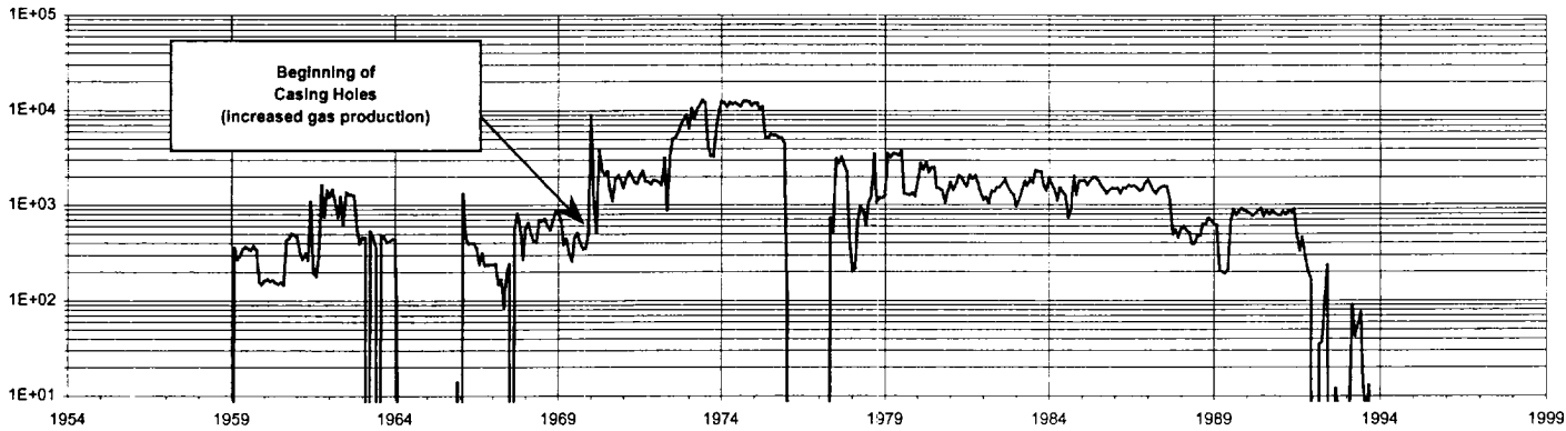
Gas Production (MCFPM)
