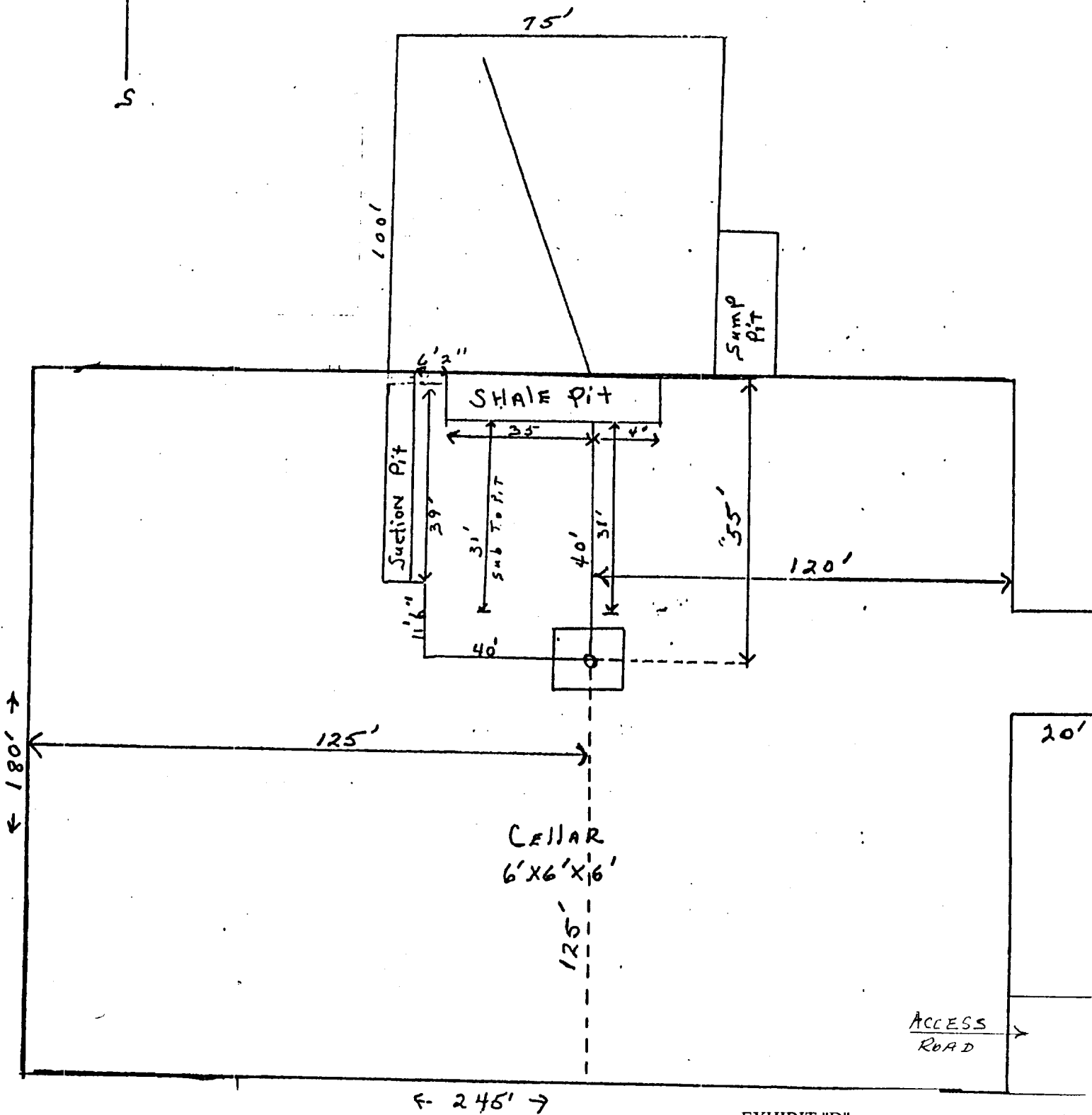
EXHIBIT "D" READ & STEVENS, INC. Truman 9 Federal, Well No. 1 Pad & Pit Layout
