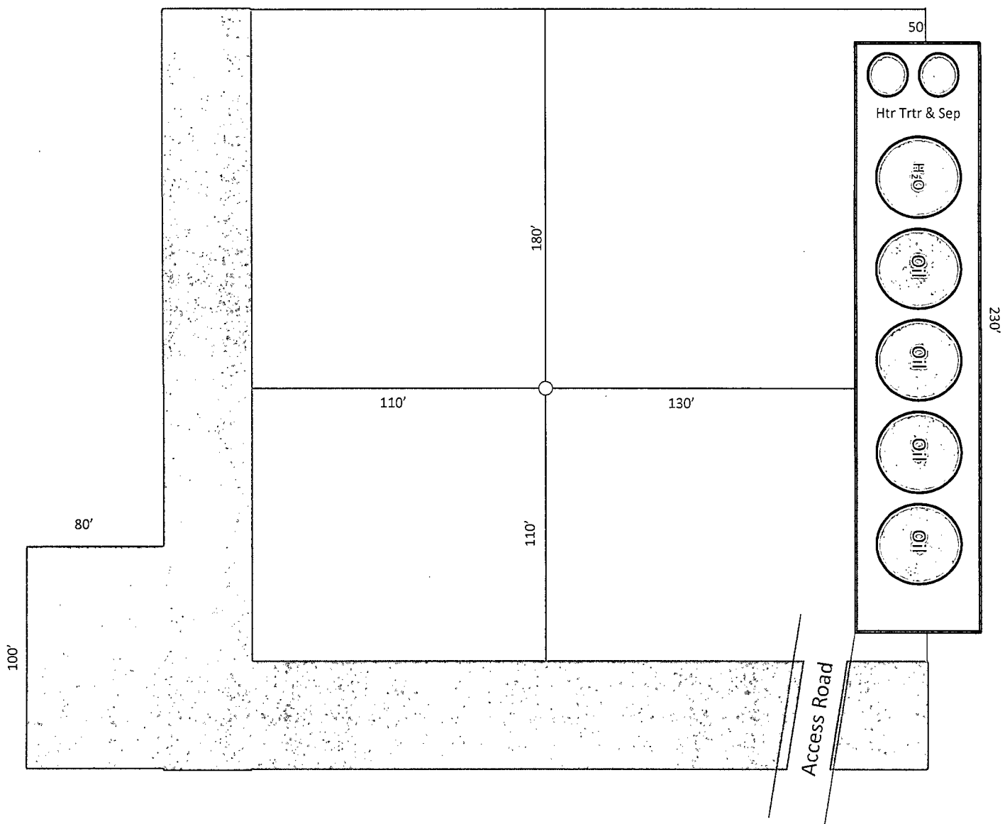
Exhibit D-1 Production Facilities and Interim Reclamation Diagram West Grama Ridge 6 Federal #4H Cimarex Energy Co. of Colorado SHL 6-22S-34E; 330 FNL & 660 FEL BHL 6-22S-34E; 330 FSL & 660 FEL Lea County, NM
