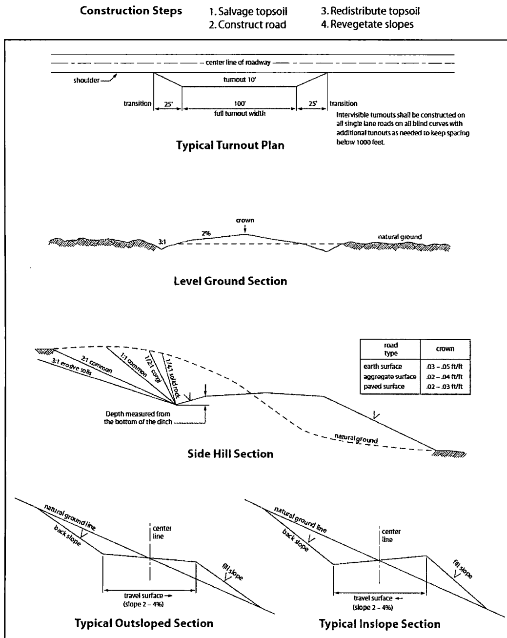
Figure 1. Cross-sections and plans for typical road sections representative of BLM resource or FS local and higher-class roads.
