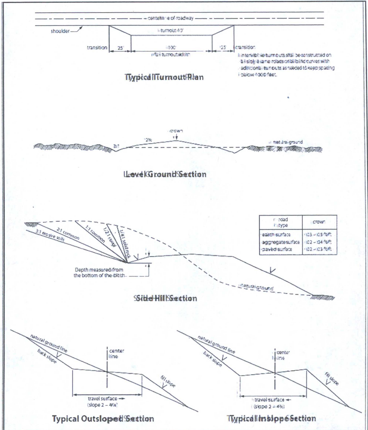
Figure 1. Cross-sections and plans for typical road sections representative of BLM resource or F&B local and higher-class roads.
