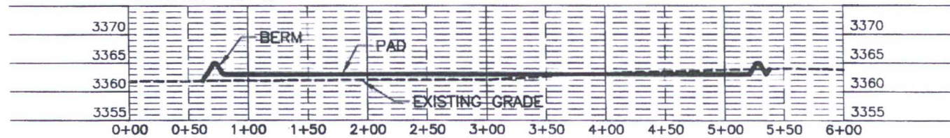
SECTION B-B'
