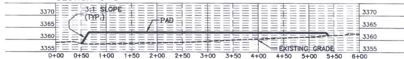
SECTION C-C'
