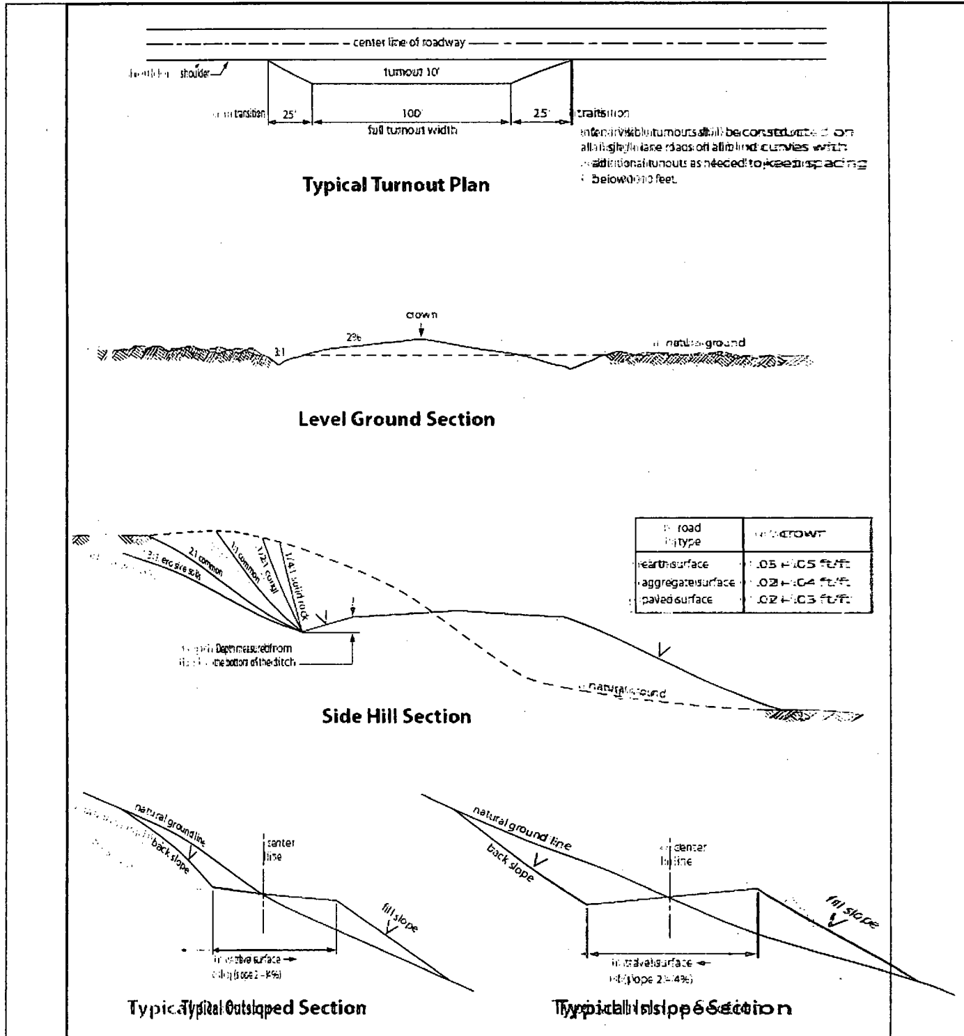
Figure 1: Cross-section and plan for typical road sections representative of IBLM resource of F5 total and high/low-class roads.
