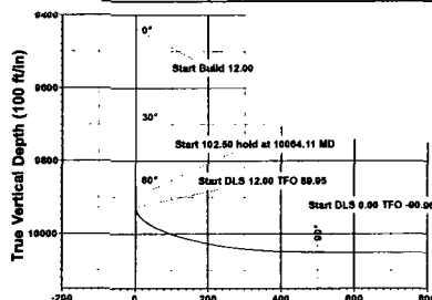
Vertical Section at 359.80° (100 ft/in)
