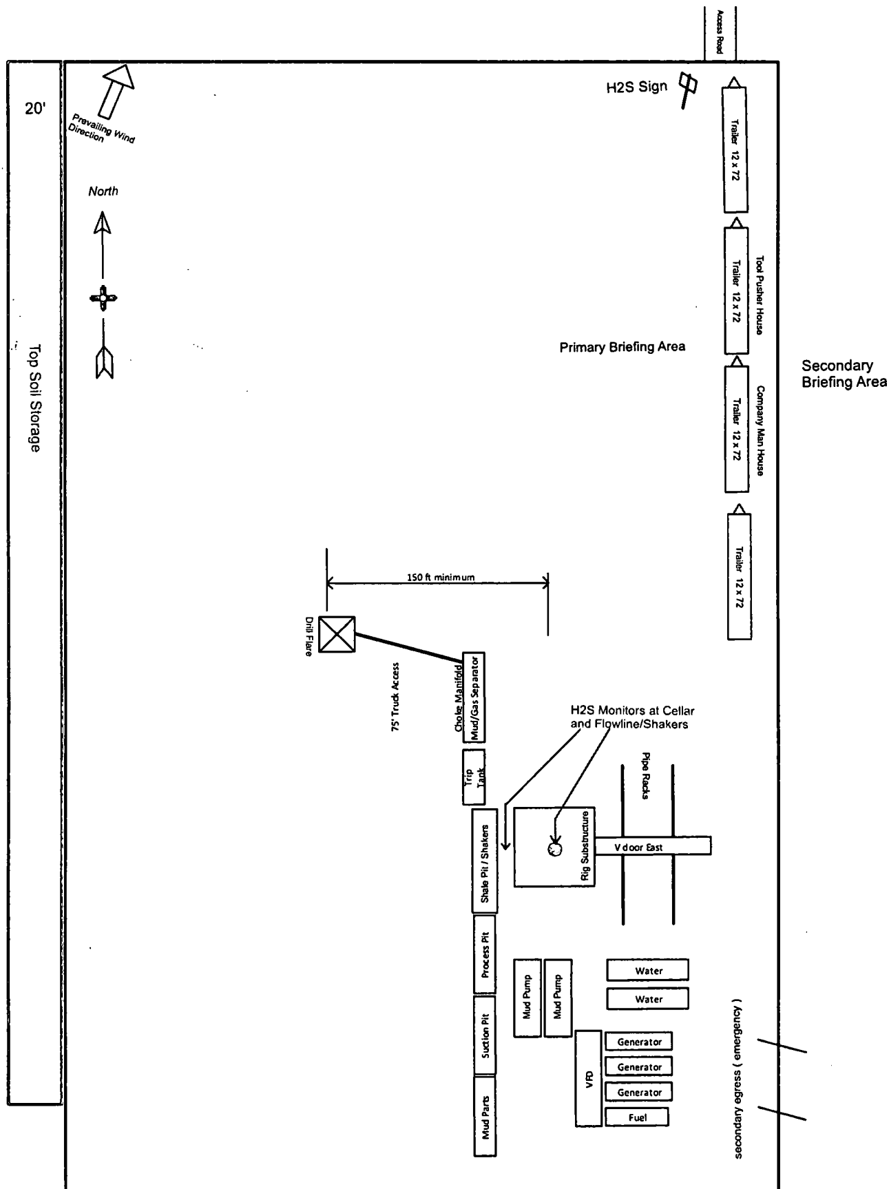
General Drill Site Layout
