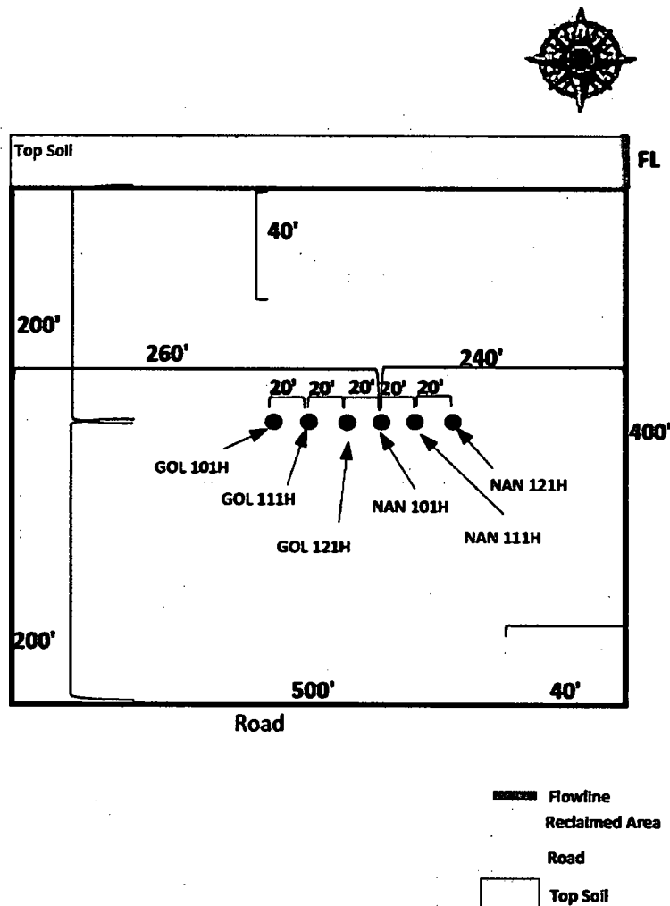
Exhibit 3 – Well Site Diagram
