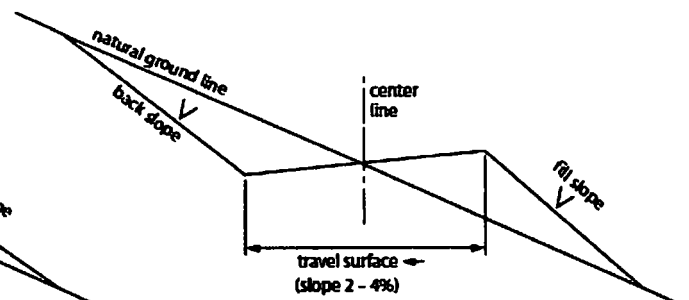
Typical Inslowed Section
