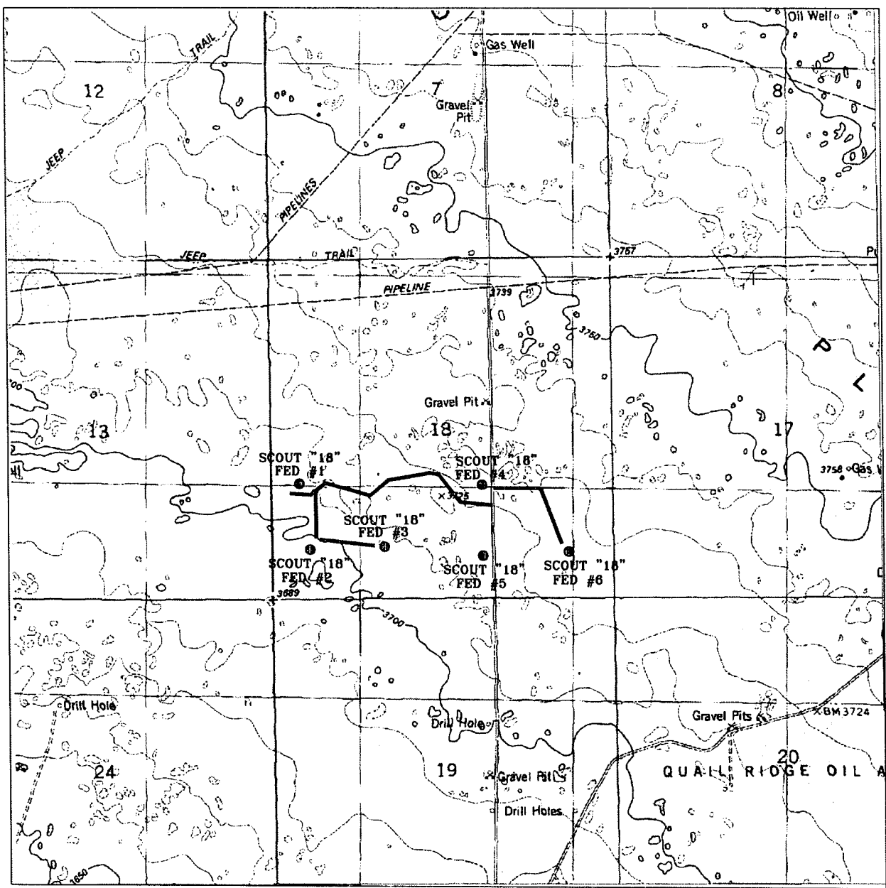
PIPELINE WELLS - PROPOSED ROAD PLAT Section 18 Township 19 South, Range 34 East, N.M.P.M., LEA County, New Mexico.
