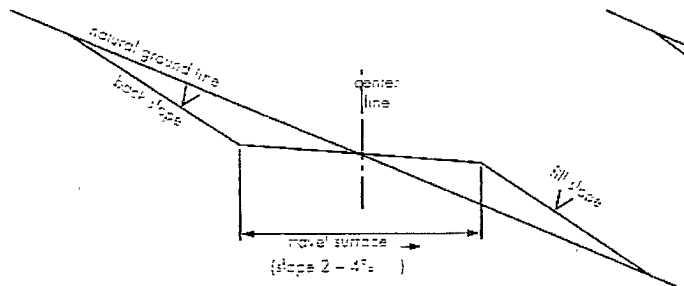
Typical Outsloped Section
