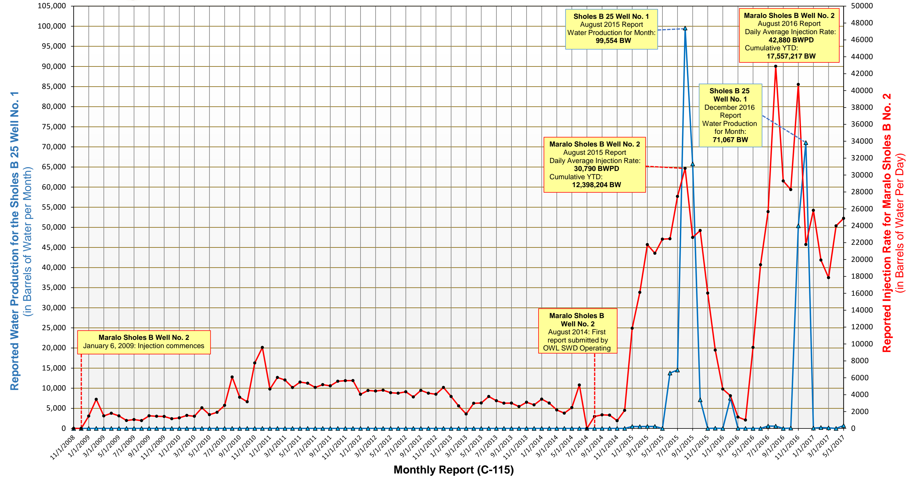
CASE NO. 15723 Division Exhibit No. 5: Graph Showing Water Production of Sholes B 25 Well No. 1 and Water Injection of Maralo B Sholes Well No. 2 vs. Time
