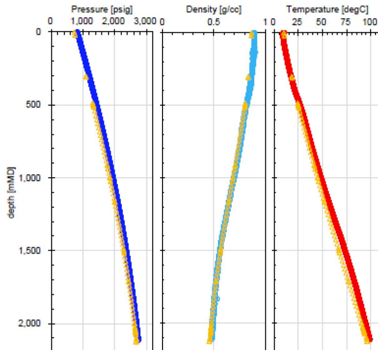
Figure 5—Pressure and temperature as a function of measured depth obtained with PLT during CO 2 injection. Blue, light-blue, and red represent observed pressure, fluid density, and temperature, respectively, while yellow triangles represent those obtained from simulations.
