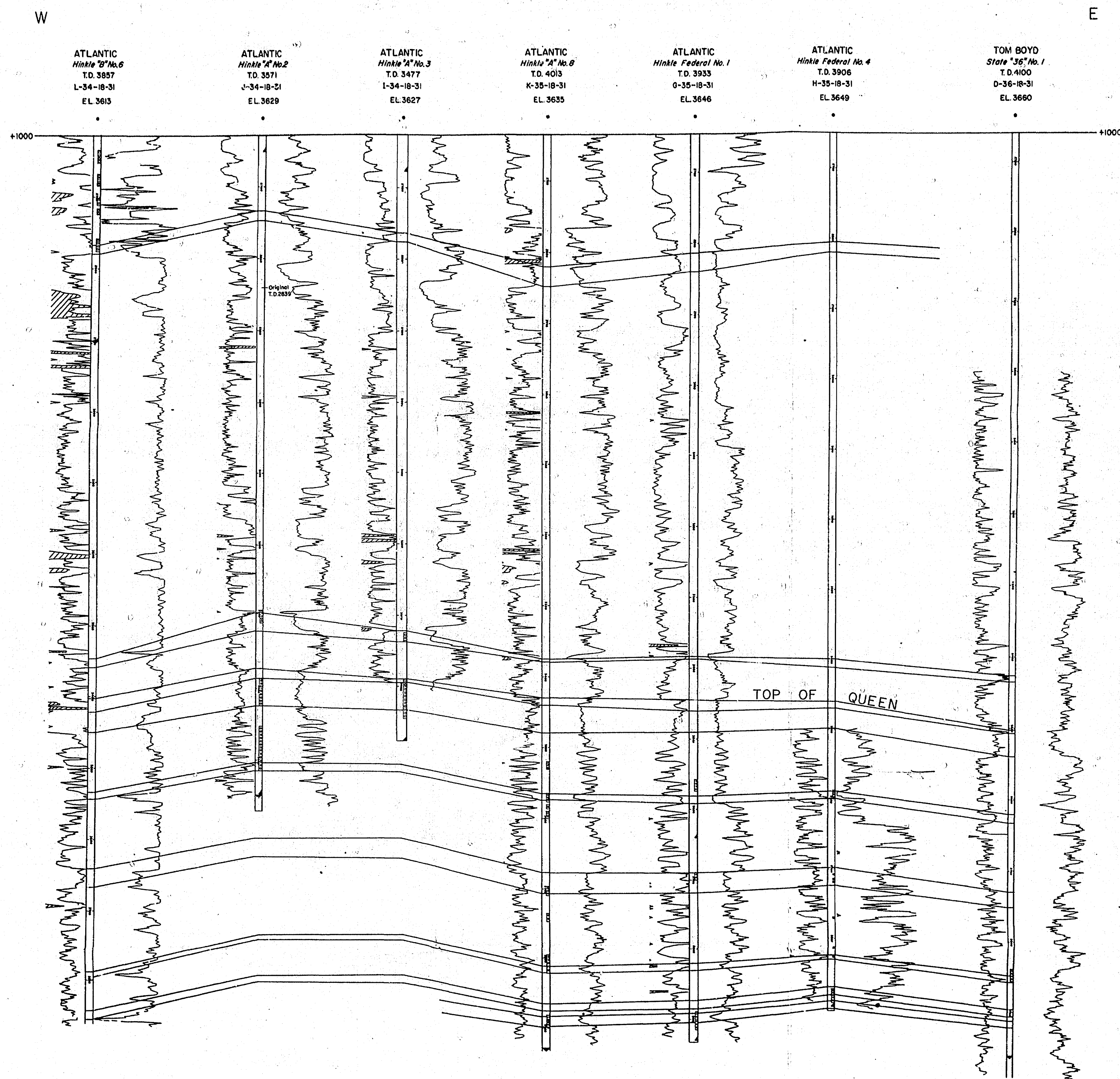
WEST-EAST CROSS-SECTION PART OF SHUGART POOL EDDY COUNTY, NEW MEXICO NO HORIZONTAL SCALE THE ATLANTIC REFINING COMPANY
