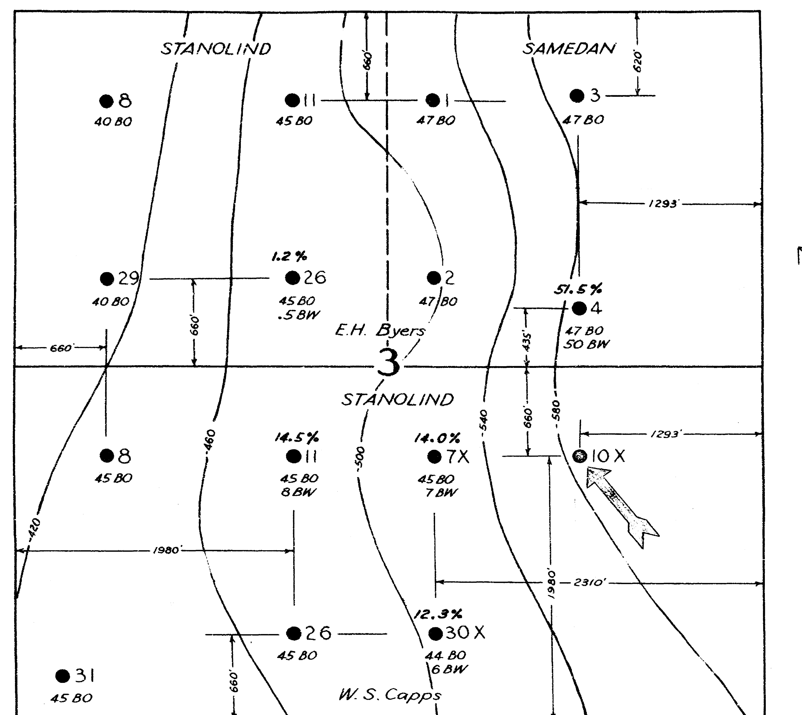
EXHIBIT "A" SEC. 3, T-19-S, R-38-E, HOBBS FIELD, LEA CO., N. MEX. Scale: 1" = 400' Drn: R.L.G. Feb. 2, 1945.
