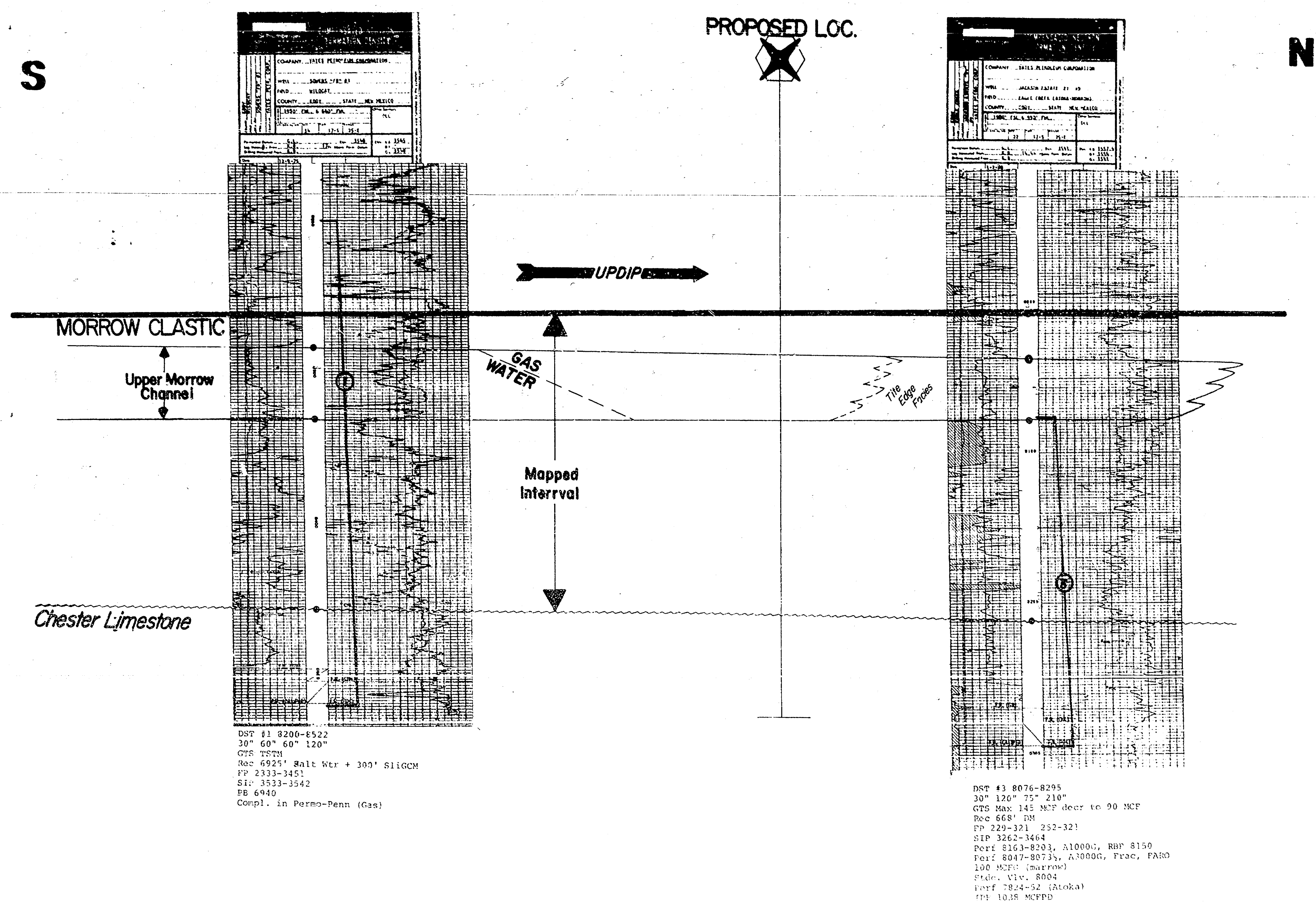
EXHIBIT 43 Crosssection
