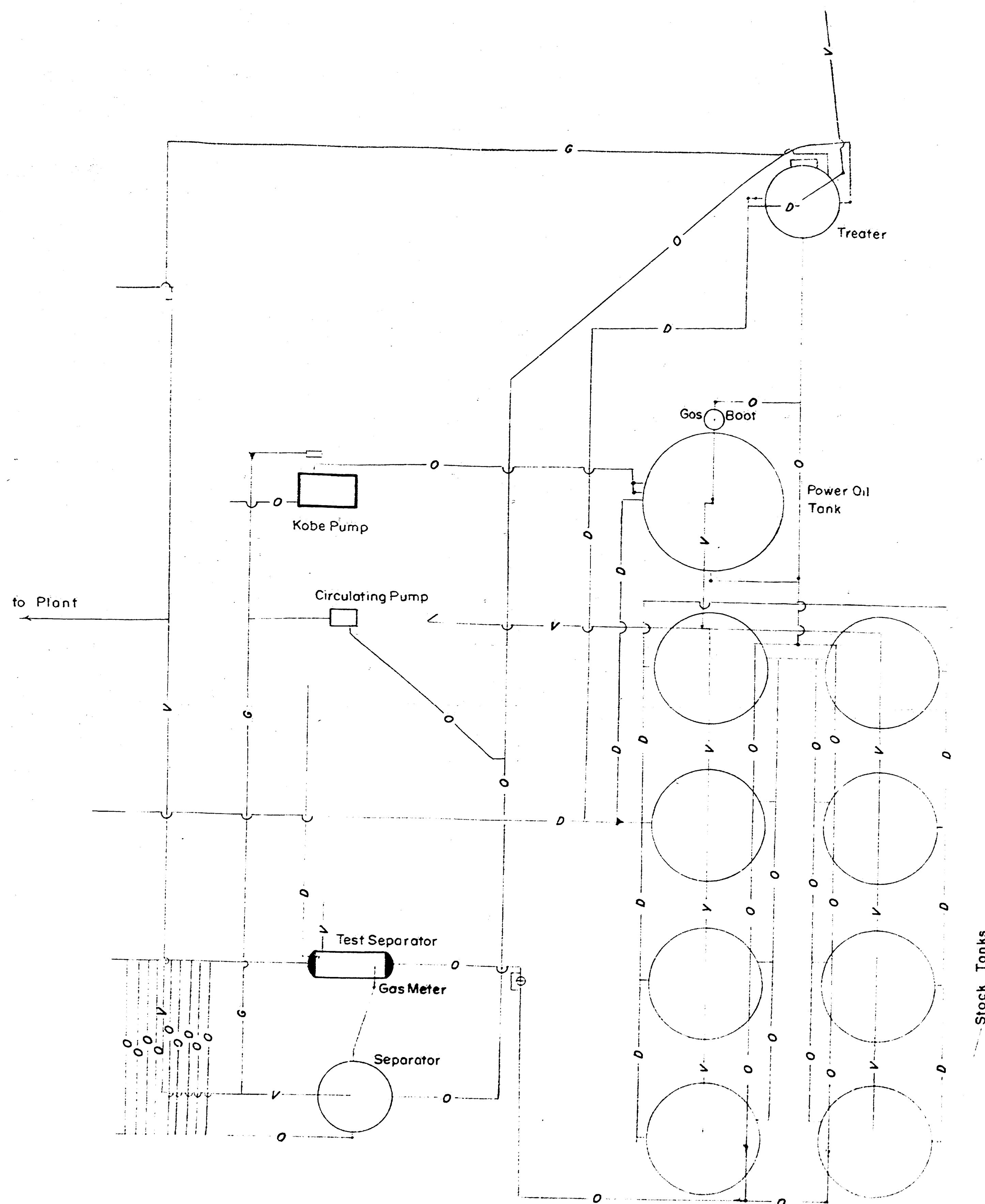
ANDERSON RANCH UNIT - WOLFCAMP Battery Detail
