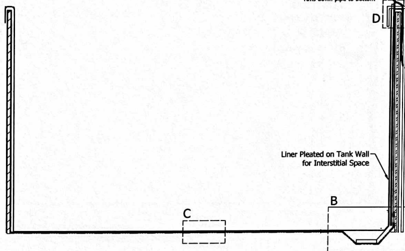
VIEW A-A TANK DETAIL
