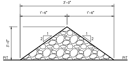
SECTION D-D NOT TO SCALE
