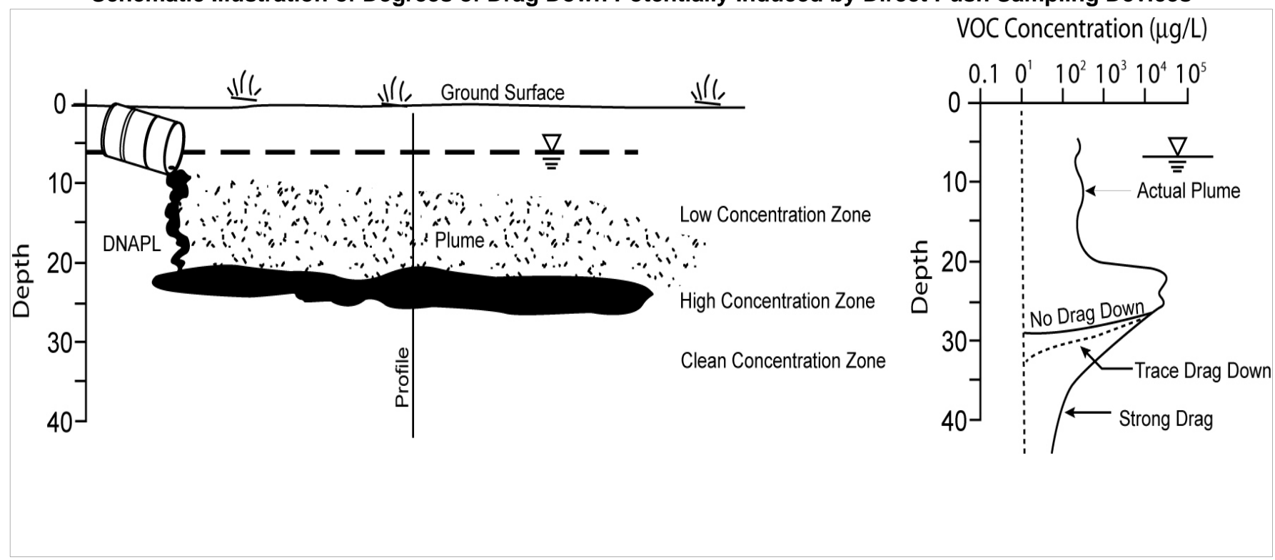
Figure 2.3 Schematic Illustration of Degrees of Drag Down Potentially Induced by Direct Push Sampling Devices
