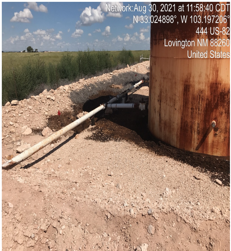
View North – Origin of spill. Cause of the release is due to corrosion on associated piping. Note a portion of the spill flow path (dark brown staining) within the release footprint.
