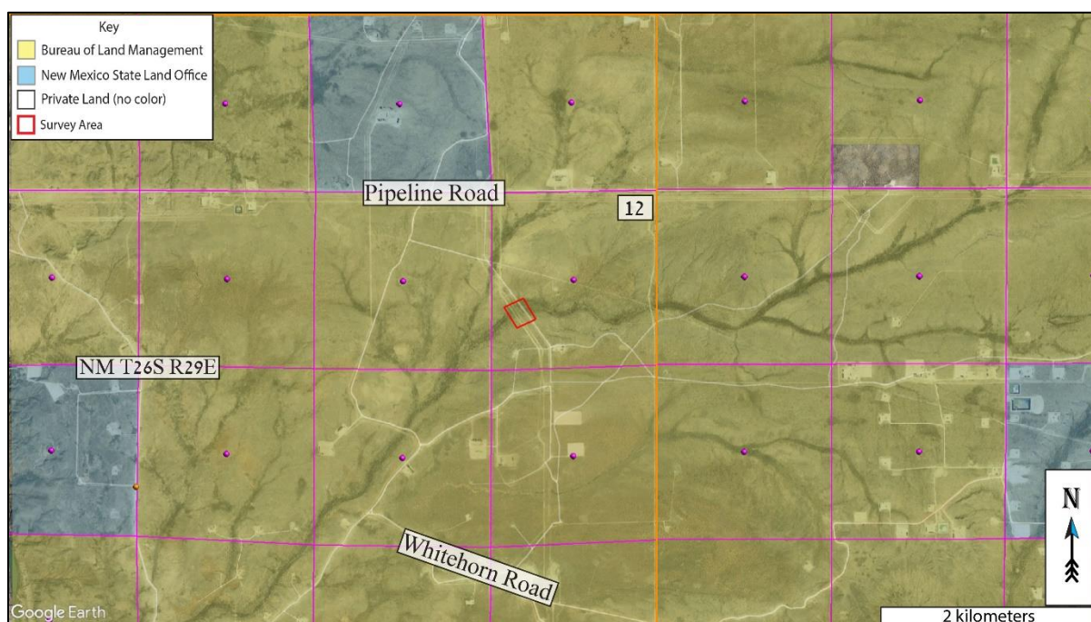
Figure 2: Land ownership [6] and PLSS [3] overview. Background image credit: Google Earth. Image date: December 21, 2019. Image datum: WGS-84.
