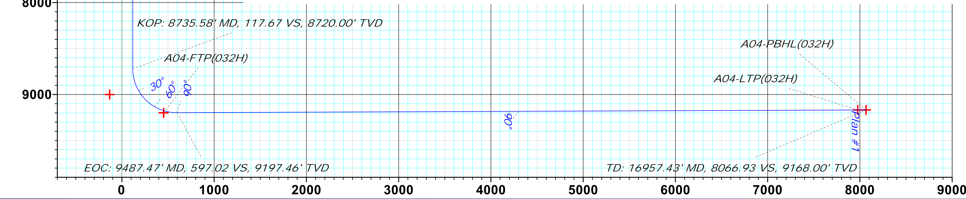
Vertical Section at 179.42° (500 usft/in)
