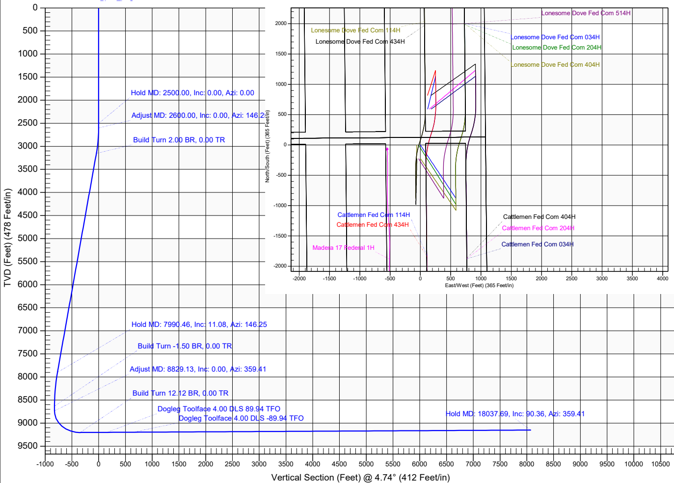
Vertical Section (Feet) @ 4.74° (412 Feet/in)
