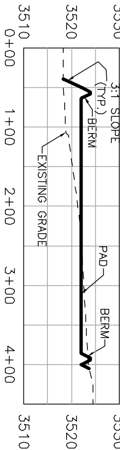
SECTION B-B
