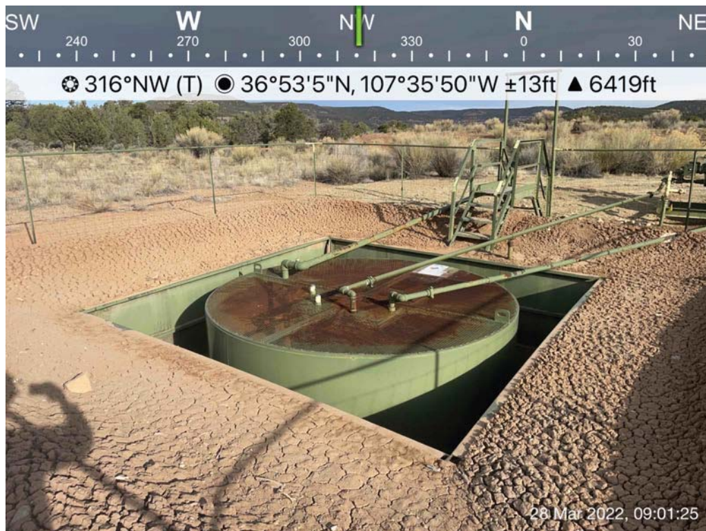
Photo 2: 80 bbls steel tank prior to removal, 3/28/2022.
