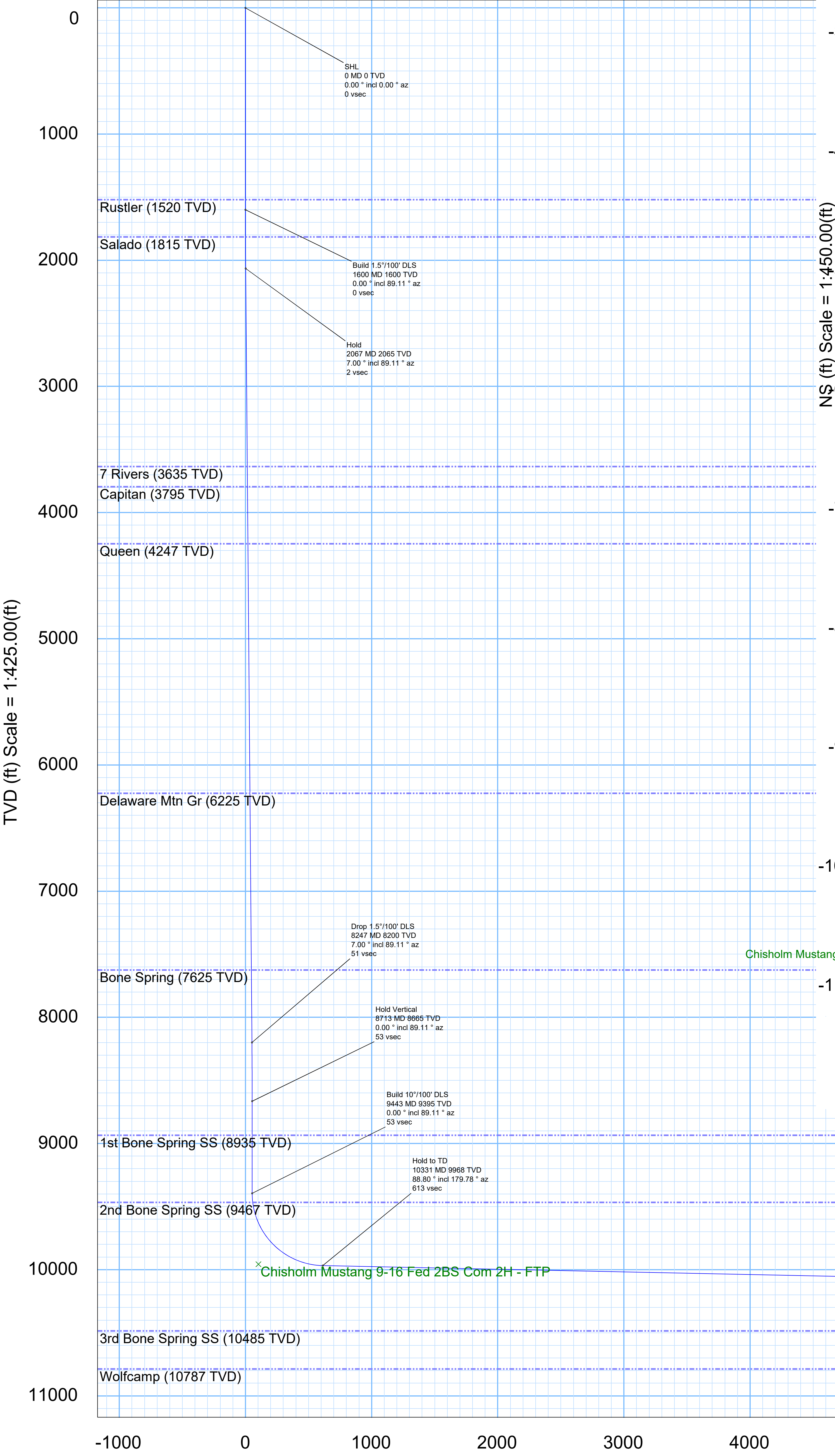
Vertical Section (ft) Azim = 175.33° Scale = 1:425.00(ft) Origin = 0N/-S, 0E/-W
