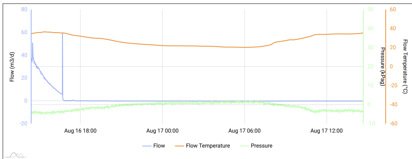
Image 3.1 – Twin Lakes SAU #025 (30-005-60334) Methane Flow/Pressure/Temperature Timeseries
