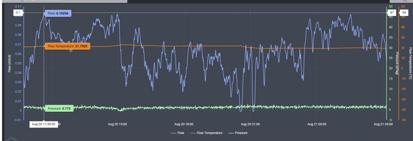
Image 4.1 – Twin Lakes SAU #011 (30-005-60571) Methane Flow/Pressure/Temperature Timeseries &amp; Peak Flow
