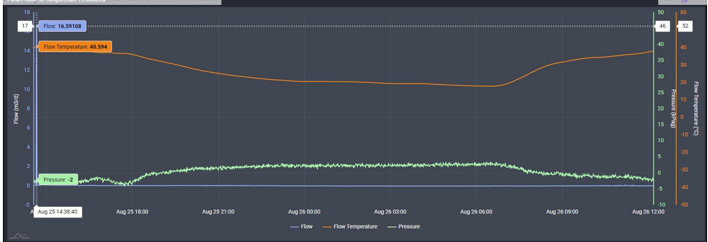
Image 4.1 – Twin Lakes SAU #108 (30-005-61334) Methane Flow/Pressure/Temperature Timeseries &amp; Peak Flow
