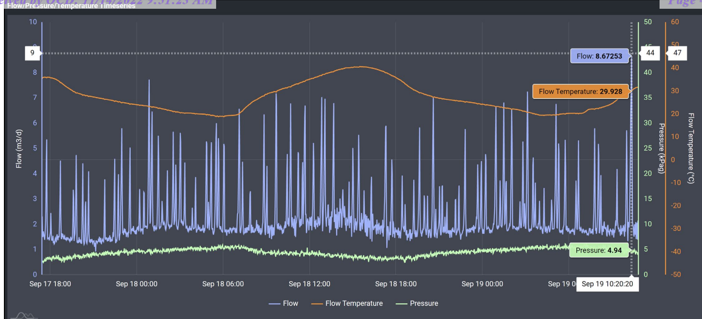
Image 4.1 – Judy #001 (30-025-24641) Methane Flow/Pressure/Temperature Timeseries &amp; Peak Flow
