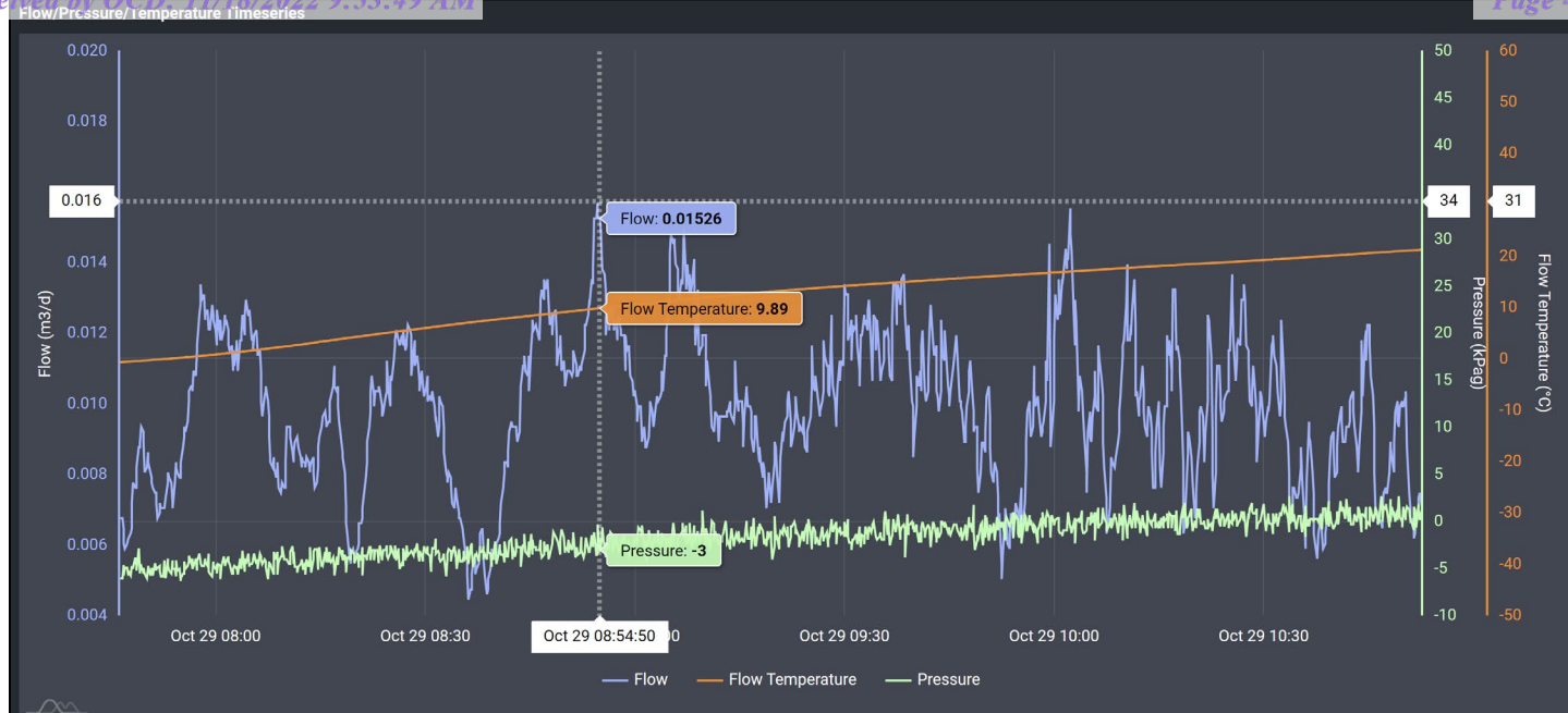
Image 4.1 – Schwalbe #001 (30-025-20472) Methane Flow/Pressure/Temperature Timeseries &amp; Peak Flow
